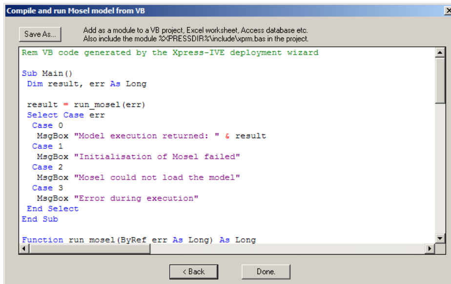
Figure 9.2: Code preview
