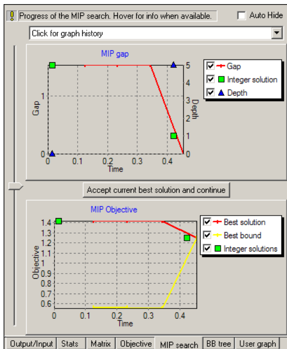
Figure 7.4: MIQP solutions
