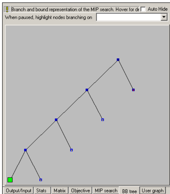
Figure 6.4: Branch-and-Bound tree
